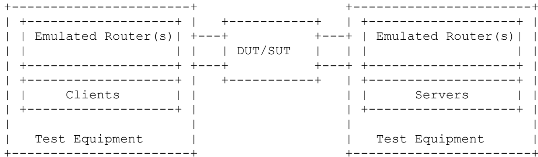
Figure 1: Testbed Setup
